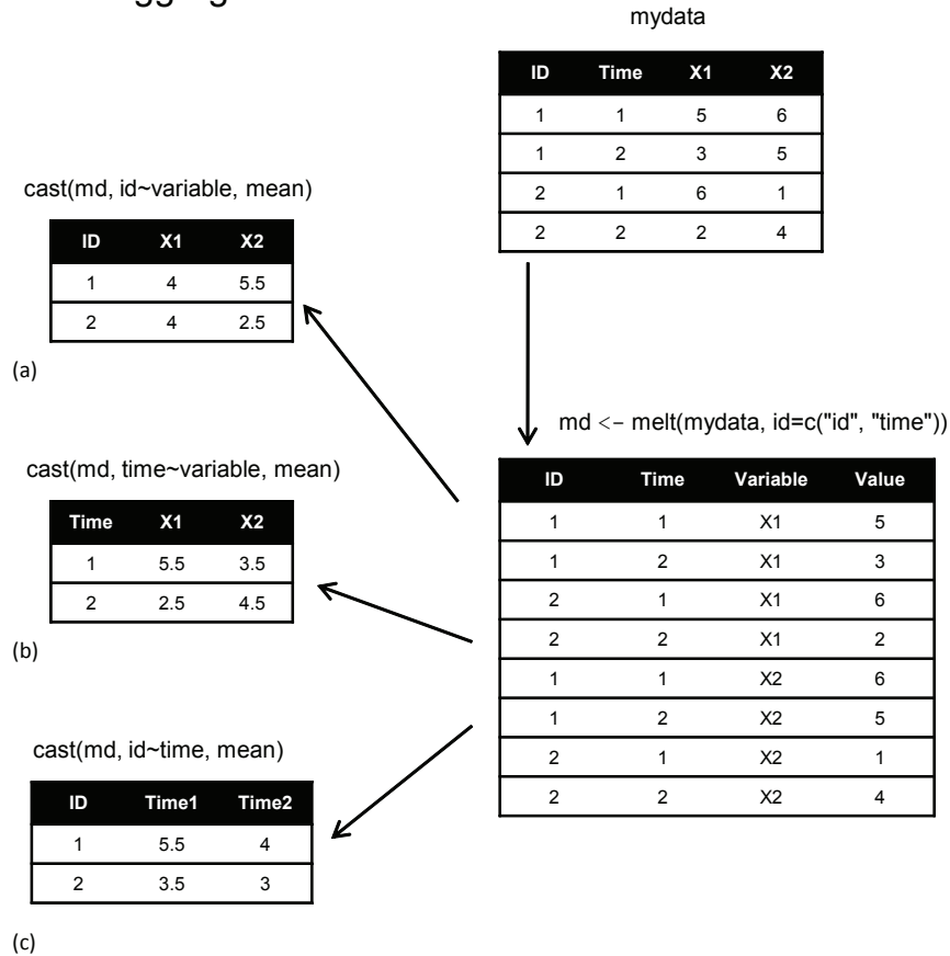
Figure 5.1 Reshaping data with the melt() and cast() functions
