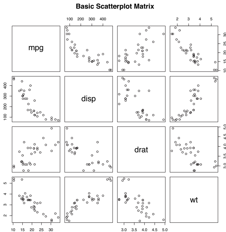
Figure 11.3 Scatter plot matrix created by the pairs() function
