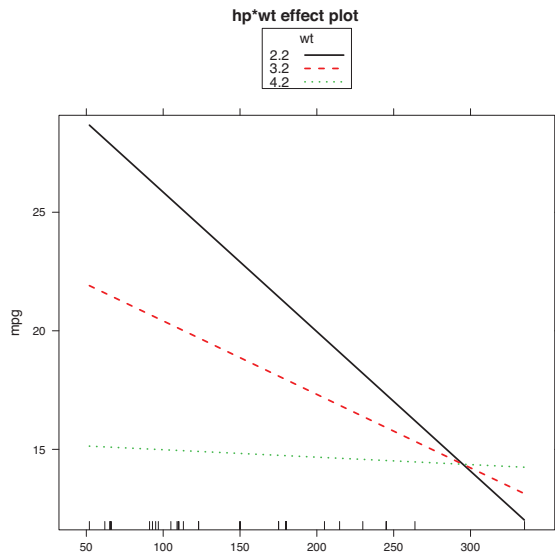
Figure 8.5 Interaction plot for hp*wt . This plot displays the relationship between mpg and hp at 3 values of wt.
