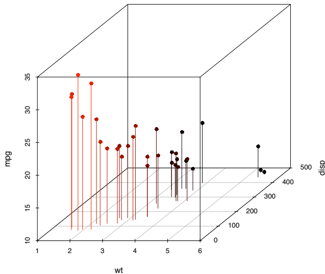
Figure 11.12 3D scatter plot with vertical lines and shading
