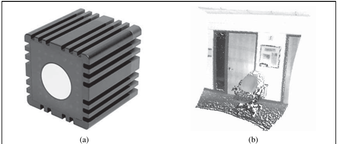
Figure 25.3 (a) Time of flight camera; image courtesy of Mesa Imaging GmbH. (b) 3D range image obtained with this camera. The range image makes it possible to detect obstacles and objects in a robot's vicinity.
