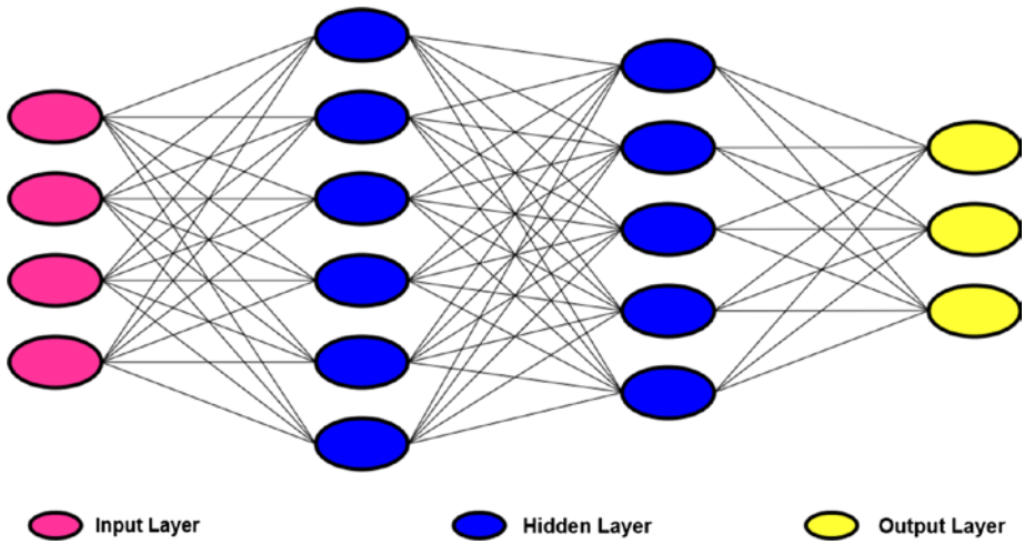
Figure 3-2. Neural network
