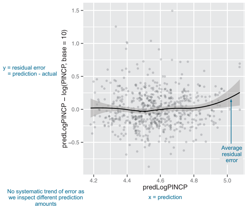
Figure 7.5 Plot of residual error as a function of prediction
