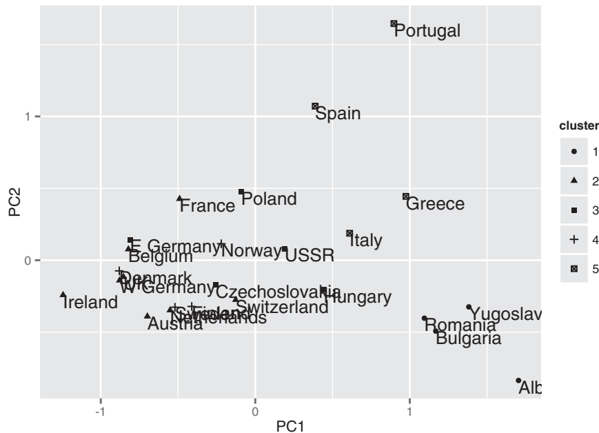
Figure 8.3 Plot of countries clustered by protein consumption, projected onto first two principal components
