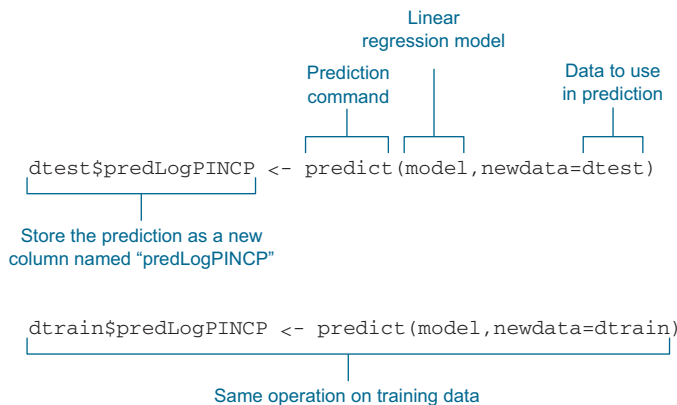
Figure 7.3 Making predictions with a linear regression model
