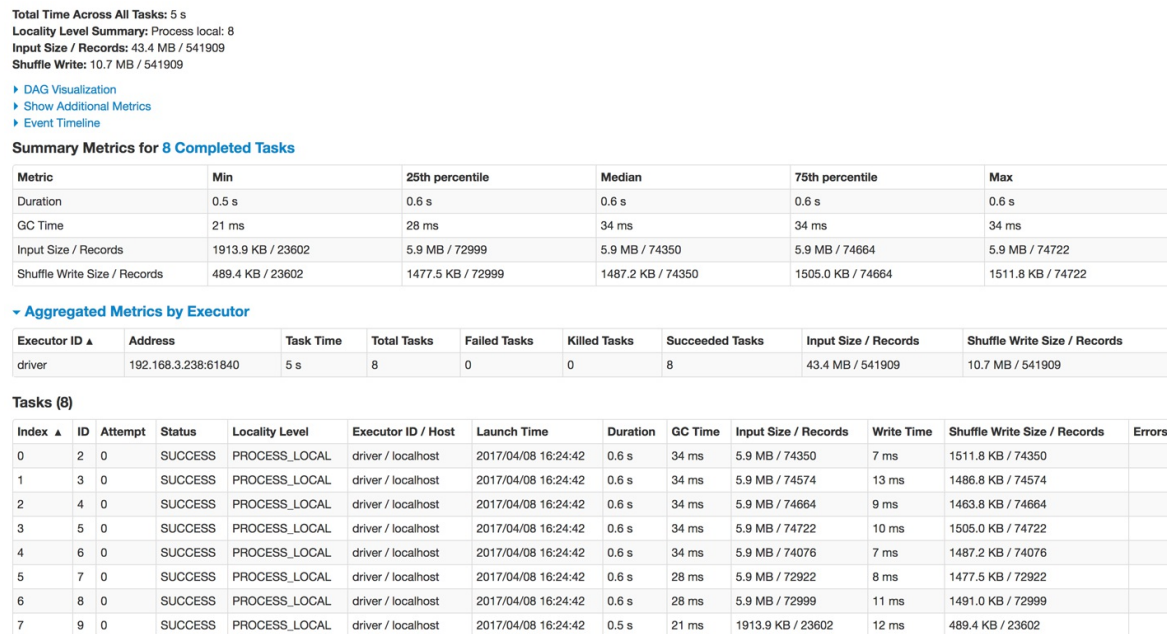
Figure 18-8. Spark tasks
