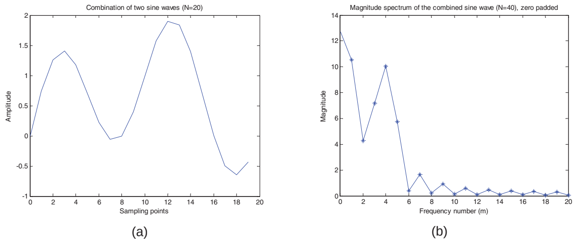
Figure 3.13: Combined sine wave (a) for length N=20 (b) spectral magnitude with 20 padded zeros.
