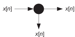
Figure 2.9: Branching operation.
