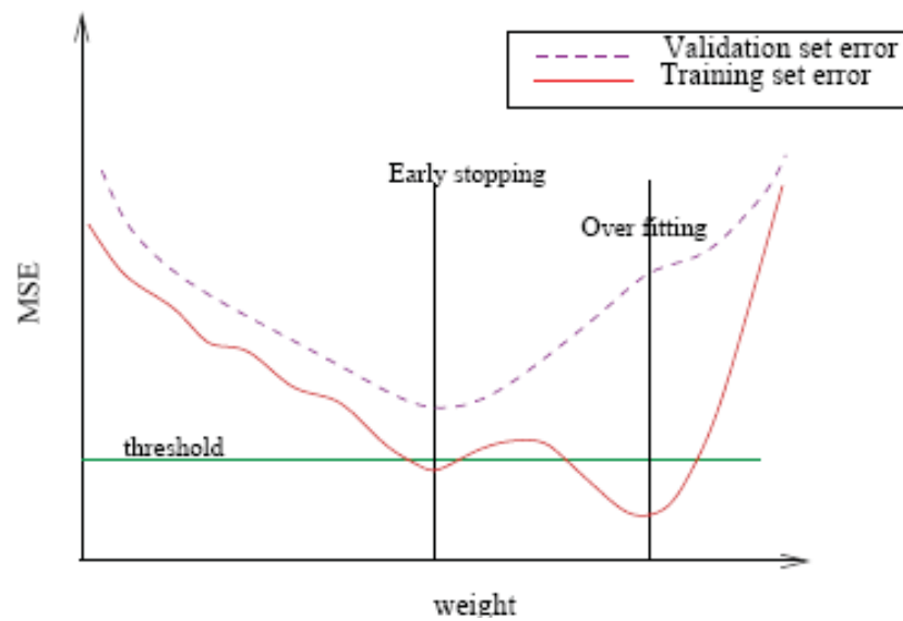
Figure 6.15: Early stopping.
