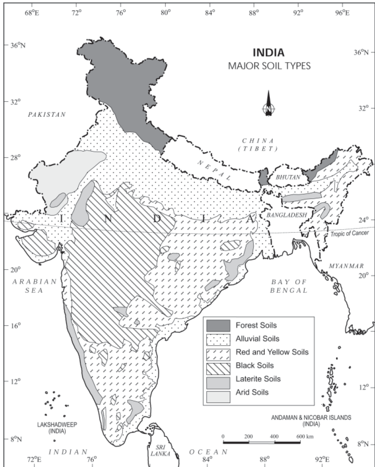
Figure 6.2 : Major Soil Types of India
