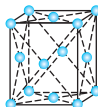
Face-centred
