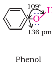
Fig. 11.1: Structures of methanol, phenol and methoxymethane
