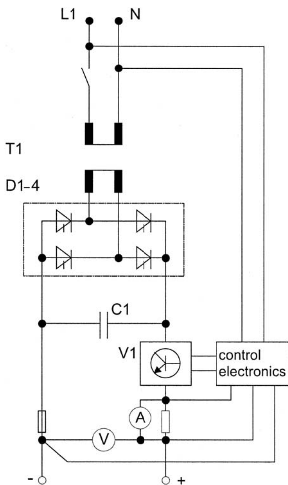
Figure 13.8 Transistor controlled charges.
