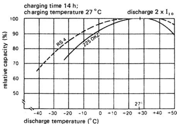
Figure 16.6 Available capacity of NiCd cells when discharged with twice the nominal current vs. temperature range (RS 4 = cell with sintered electrodes; 225 DKZ = cell with mass electrodes).
