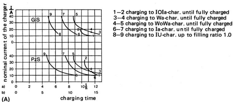
Figure 12.3 Charging time for lead-acid and NiCd batteries. (A) Rectifier nominal current for charging traction lead-acid cells GiS and PzS at 20°C (68°F) after discharge of (a) 80% and (b) 100% of C_5 . (B) Rectifier nominal current for charging of stationary lead-acid cells OPzS, Gro, GroE at 20°C per 100 Ah K_5 after discharge of (a) 80% and (b) 100% of C_5 (operation conforming to DIN 40729). (C) Rectifier nominal current for charging R-, TN/TS-, and F-type cells at 20°C per 100 Ah C_5 after discharge of (a) 80% and (b) 100% of C_5 (operation conforming to DIN 40729).
