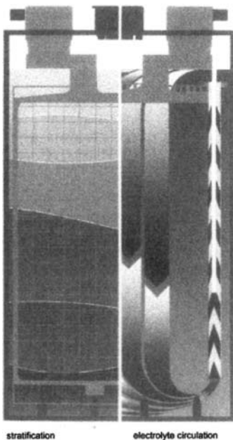
Figure 2.10 The principle of electrolyte circulation.
