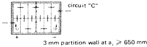
Figure 2.1 Circuits of 24-V traction batteries to DIN 43 535.
