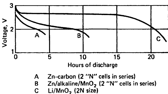
Figure 18.9 Discharge graph of old and new primary batteries: A = Leclanché, B = alkaline, C = lithium/manganese dioxide. (From Ref. 3.)
