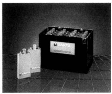
Figure 4.12 Battery module with nickel/metal hydride cells and performance data.
