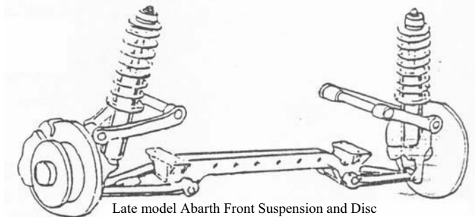
Late model Abarth Front Suspension and Disc Brakes. Special alloy cross-member, lower A-arms, and coil-over shocks replace the fiat transverse leaf spring.
