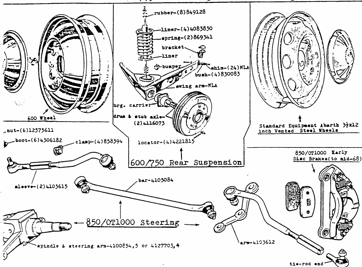
Figure 20a Standard Suspension &amp; Steering
