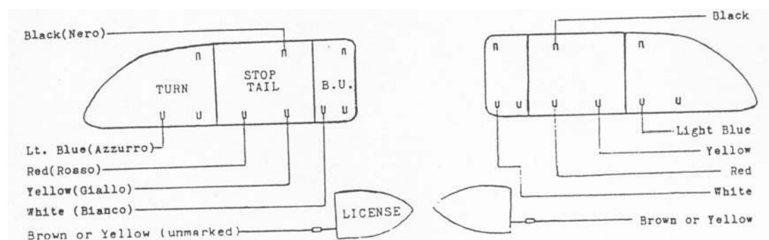
fiat 850 Sport Spider (903) 1970-72 Rear-Panel Light Wiring as been from rear(72-73 similar)
