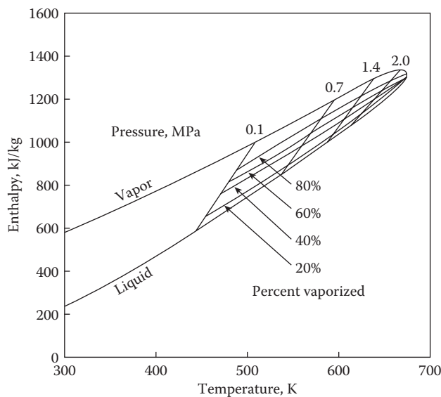
FIGURE 10.17 Enthalpy of Jet A fuel.
