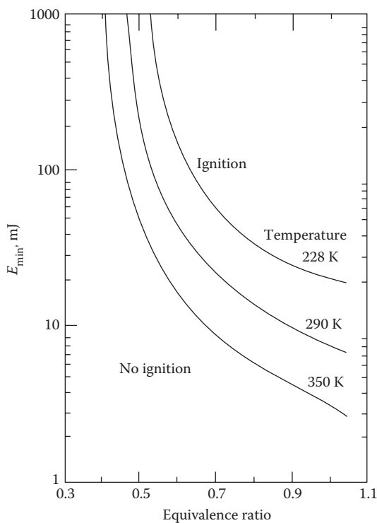
FIGURE 5.35 Effect of air temperature on minimum ignition energy; P=20 kPa, U=15 m/s, SMD=60 \mu\text{m} . (Reprinted from Ballal, D.R. and Lefebvre, A.H., Combustion and Flame , 31(2), 115–126, 1978. Copyright by The Combustion Institute.)
