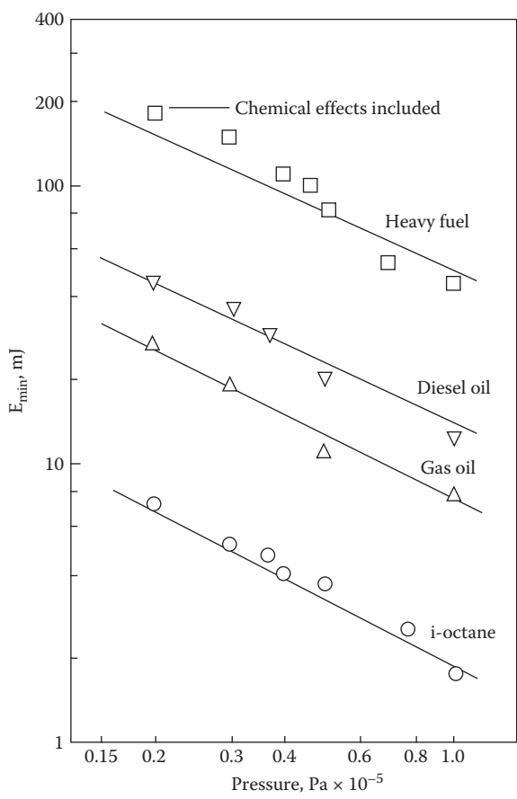
FIGURE 2.14 Improvements in correlation resulting from inclusion of chemical effects. U = 15 \text{ m/s} , \phi = 0.65 , \text{SMD} = 60 \mu\text{m} . (From Ballal, D.R. and Lefebvre, A.H., Eighteenth Symposium (International) on Combustion , The Combustion Institute, Pittsburgh, PA, 1737–46, 1981.)
