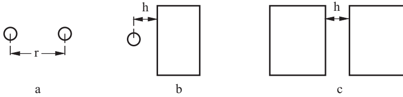
Fig. 3.1 Interaction between two atoms (a), an atom and a half-space (b) and between two half-spaces (c).
