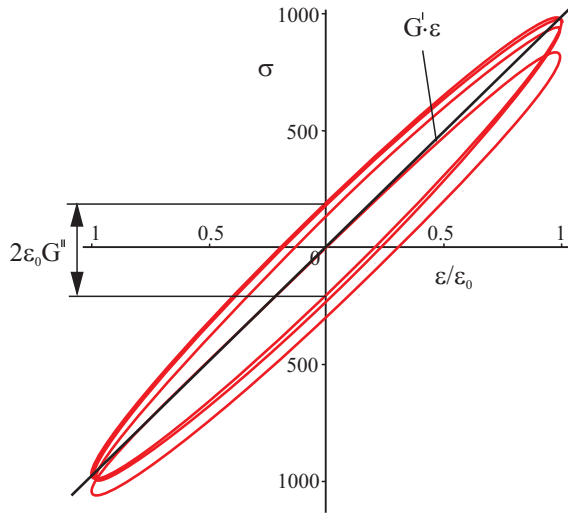
Fig. 15.6 Stress-strain diagram for a viscoelastic material.
