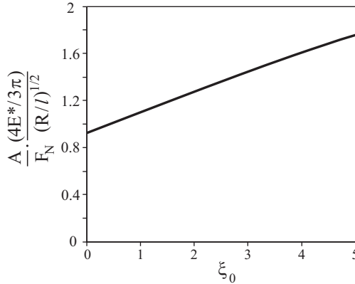
Fig. 7.4 Dependence of the ratio of contact area and compressive force on the separation variable \xi_0 .
