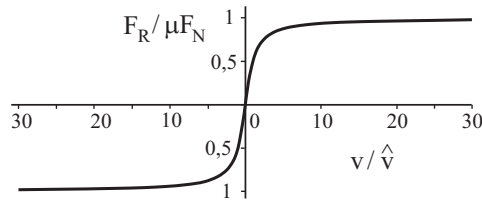
Fig. 19.1 Approximation of the law of friction by a continuous function of velocity.
