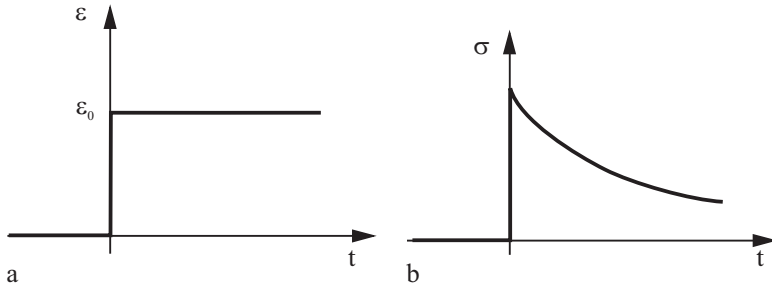
Fig. 15.3 If a rubber block is quickly deformed by \varepsilon_0 at time t = 0 , then the stress increases initially to a high level and afterwards, relaxes with time to a much lower level.
