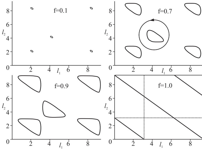
Abb. 11.11 Bifurcation sets of the potential (11.35) for various external forces f = F / U_0 k . Directional motion is possible as long as the bifurcation sets form closed forms that can be surrounded by a path without it intersecting them.
