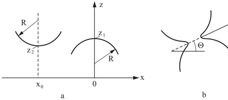
Fig. 7.15 (a) Two asperities with the same radii of curvature; (b) Asperities in contact.
