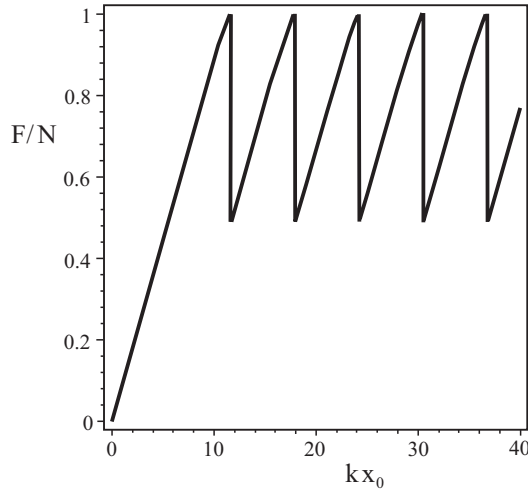
Fig. 11.7 Dependence of the force acting on the body in model (11.20) as a function of the coordinate of the sliding sled x_0 for the case c / Nk = 0.1 . Because of the emergence of elastic instabilities, the average value of the force is not equal to zero.
