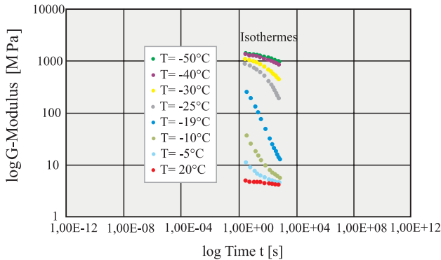
Fig. 15.12 Measurements of stress-relaxation for various temperatures in a given time window.
