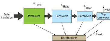
Figure 2.20 Diagram showing the transfers and transformations of energy as it flows through an ecosystem. Arrows showing flows of energy vary in width, proportional to the amount of energy being transferred
