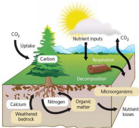
Figure 3.8 Soil systems, lithosphere systems and atmospheric systems
