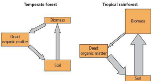
Figure 2.23 Diagrams showing the major nutrient flows and storages in two different ecosystems. The size of the boxes and width of the arrows are proportional to the size of the storages and flows they represent
