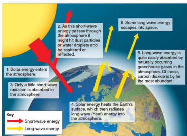
Figure 6.1 The greenhouse effect
