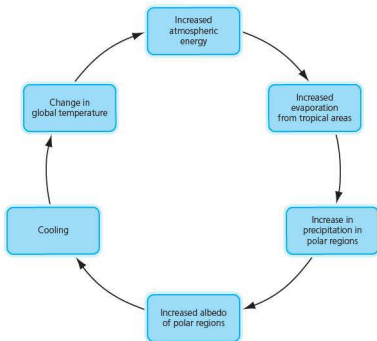
Figure 6.7 Negative feedback in global warming
