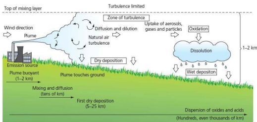
Figure 5.13 Acid deposition
