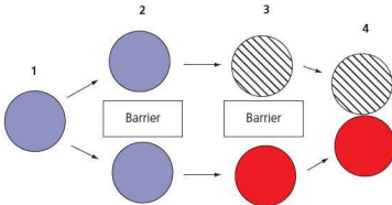
Figure 4.3 The process of speciation: 1 original population; 2 geographical isolation divides the population into two separate groups; 3 populations become adapted to different local conditions and become genetically different from each other; 4 reproductive isolation occurs and the species cannot interbreed if they meet
