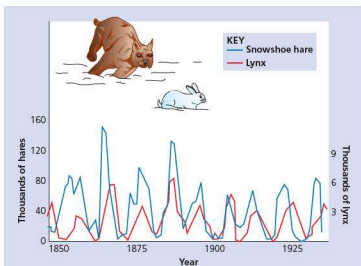
Figure 1.14 Predator–prey relationships
