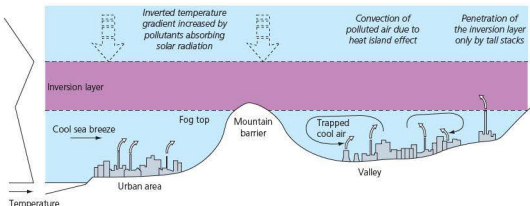
Figure 5.12 Temperature inversion
