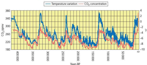
Figure 6.2 Carbon dioxide levels in geological time
