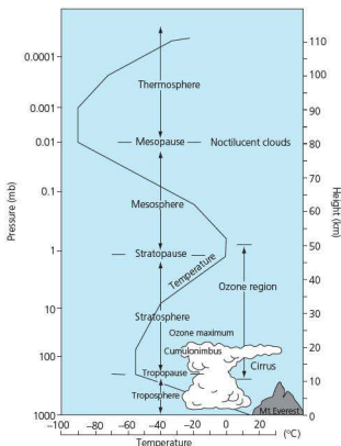
Figure 5.11 The structure of the atmosphere
