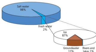
Figure 3.19 Freshwater sources
