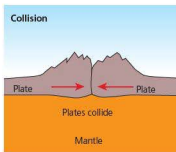
Figure 4.6 A collision plate margin: continental plates collide, leading to increased continental plate thickness and eventually new mountain ranges (e.g. the Himalayas, where the Indian plate is pushed against the Asian plate)
