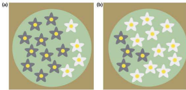
Figure 1.5 The Daisyworld model. a) Daisyworld early in its history; b) Daisyworld late in its history, after its Sun has become brighter
