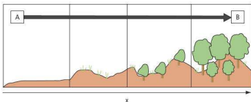
Figure 2.31 Succession in a sand dune ecosystem. The x-axis represents either time or distance from the sea. A is a pioneer community and B a climax community
