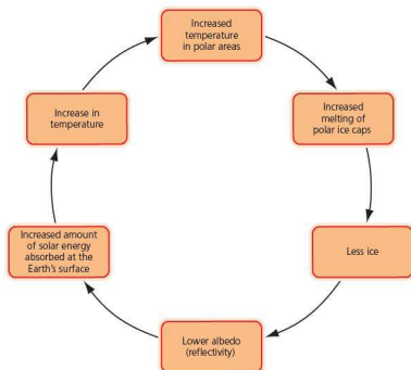
Figure 6.6 Positive feedback in global warming
