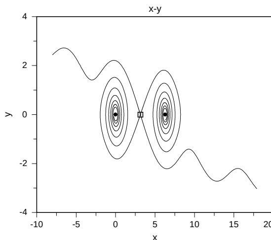
Figure 12.3: Stable and unstable separatrices at a saddle for an unforced damped pendulum. Which are the stable separatrices?
