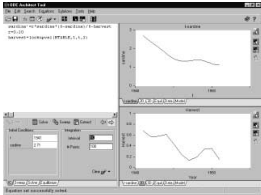
Figure 1.11: Model sardine biomass (upper), harvested biomass (lower).
