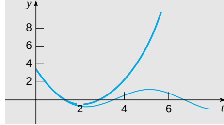
FIGURE 4.2.3 Plots of the solutions (16) (light curve) and (17) (heavy curve).
