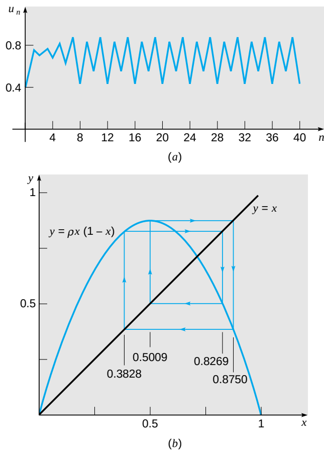
FIGURE 2.9.5 A solution of u_{n+1} = \rho u_n(1 - u_n) for \rho = 3.5 ; period four. (a) u_n versus n ; (b) a four-cycle.
