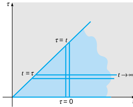
FIGURE 6.6.1 Region of integration in F(s)G(s) .
